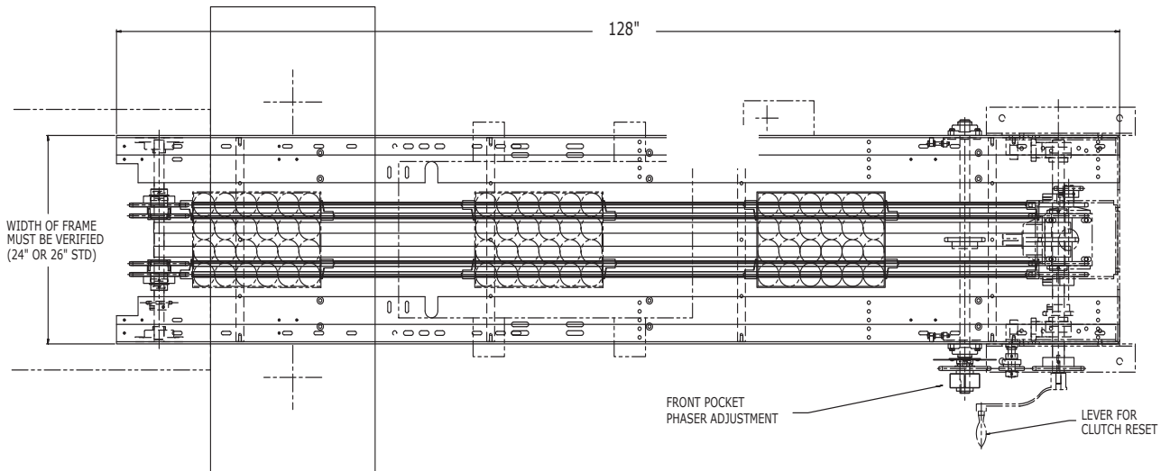
Figure 1.3 - Overhead View of New Compression Section
