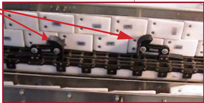
Figure 1.2 - Quick Adjusting Plastic Lugs
