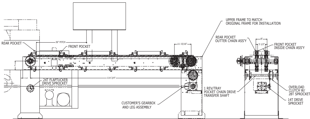
Figure 1.4 - Side View of New Compression Section
