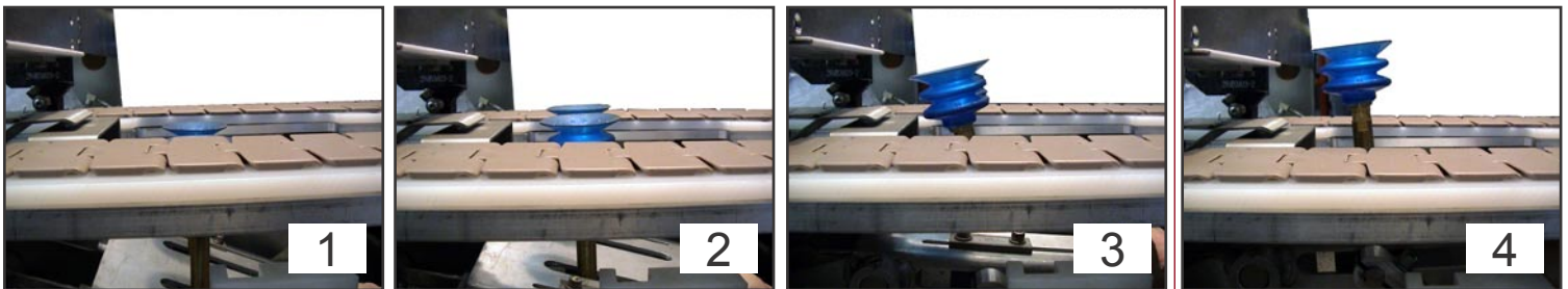
Figure 1.1 - Cam driven Vacuum Cups (Shown at four stages of motion)
